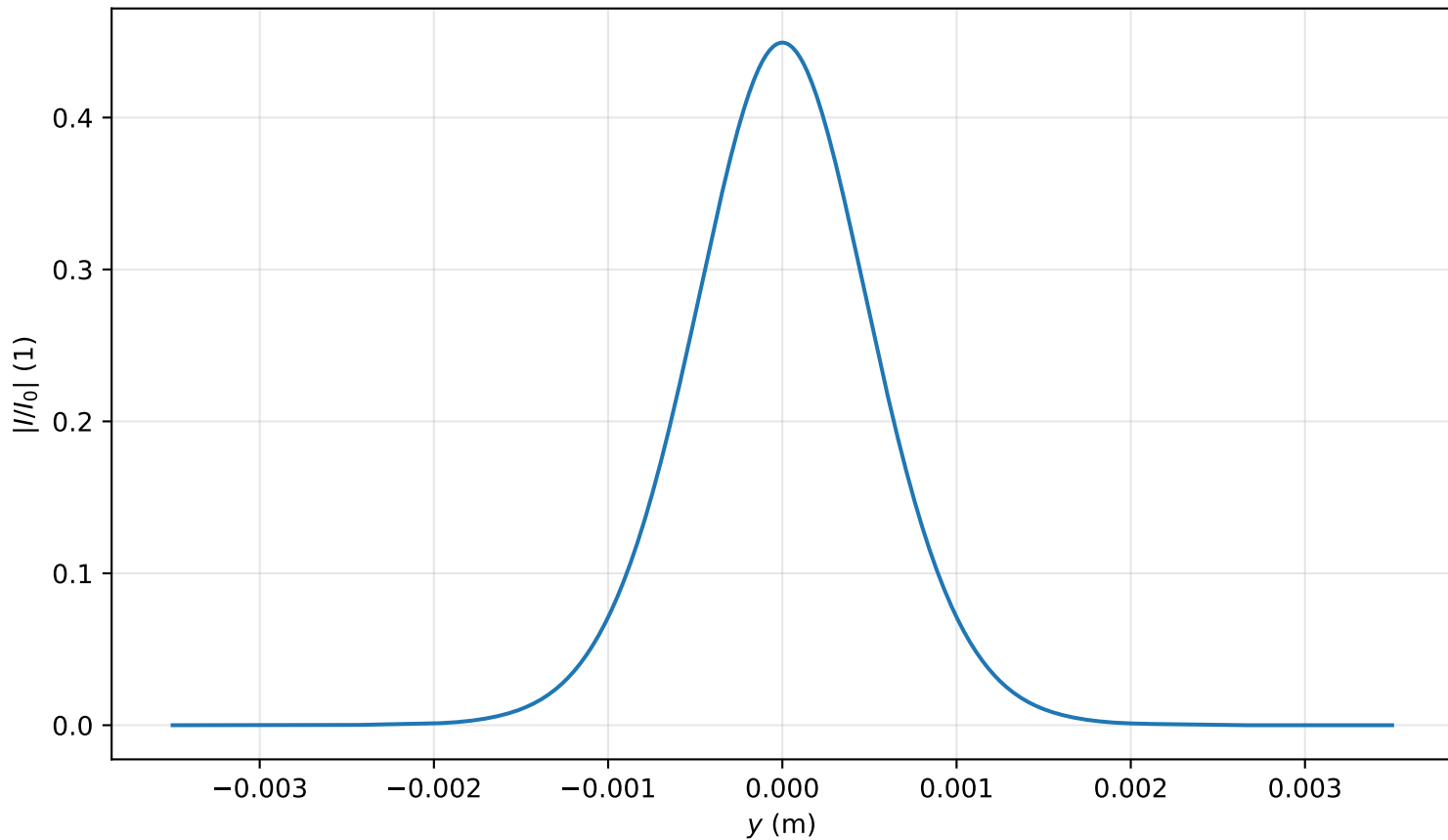
Intensity profile I(x = 0, y, z = 3.184)/I_0 , P_{in}=0.4P_{cr} , artificial time
